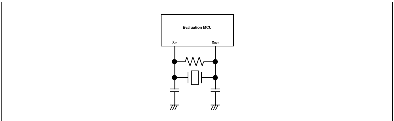
Figure 2.22 Circuit in which oscillation does not occur
